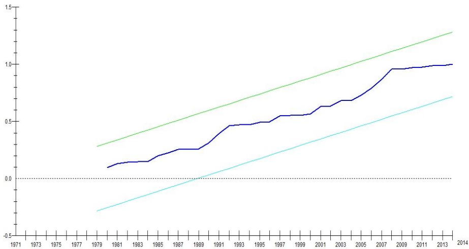
a- Plots of CUSUM Statistics for Coefficient Stability
